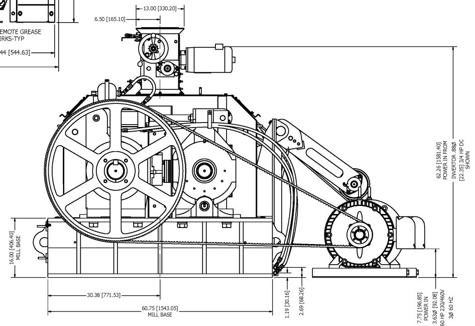
RIGHT SIDE VIEW GUARDS REMOVED
