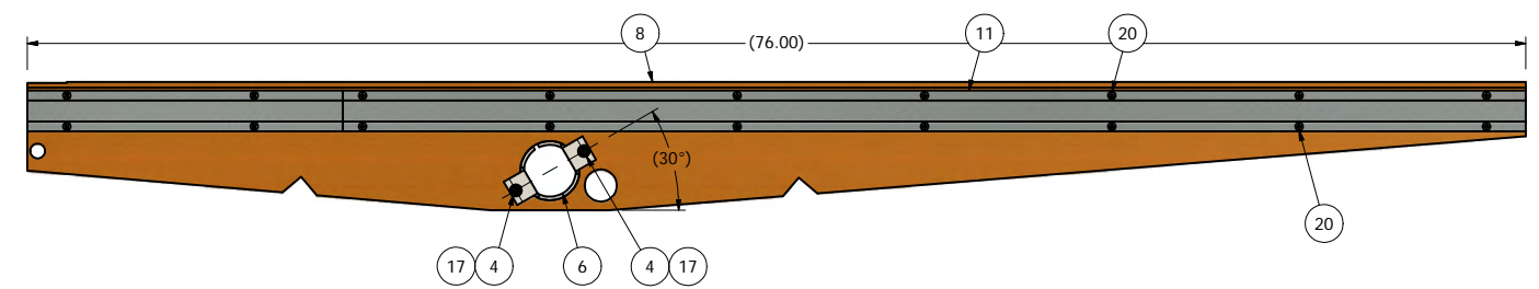
STEP 1: RIGHT ROCKER SIDE ASSEMBLY, LEFT SIDE VIEW TYPICAL ASSEMBLY FOR LEFT ROCKER SIDE
