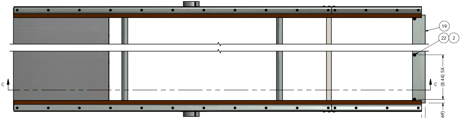
STEP 3: GIRT INSTALLATION, TOP VIEW
