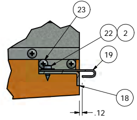
DETAIL F SCALE 1/2
