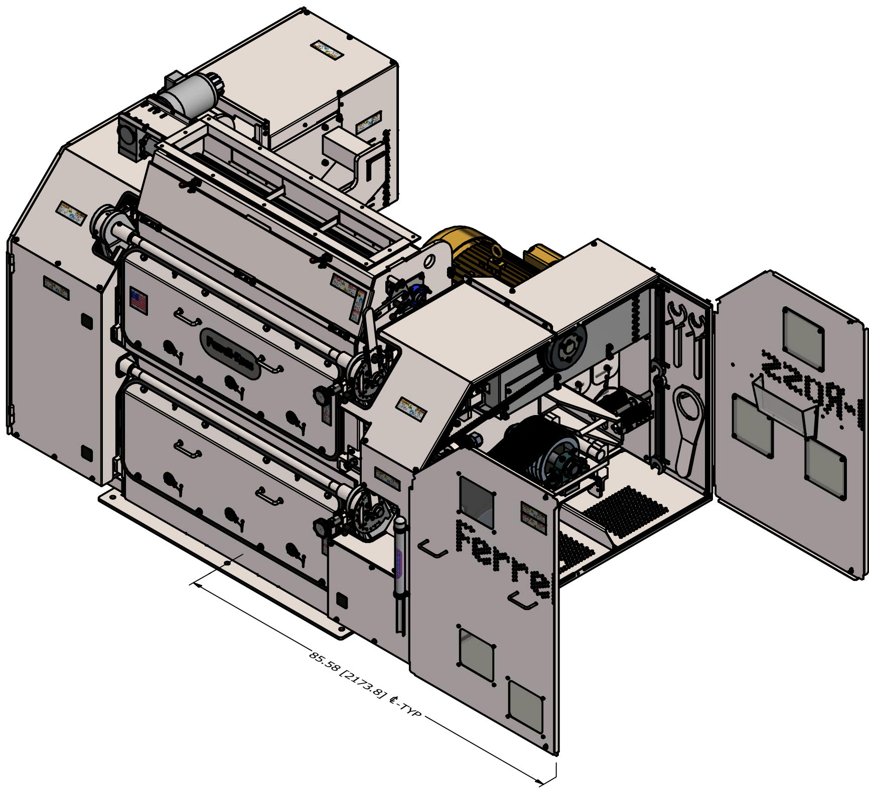
RIGHT GUARD DOORS SHOWN OPEN SCALE 0.06 : 1
