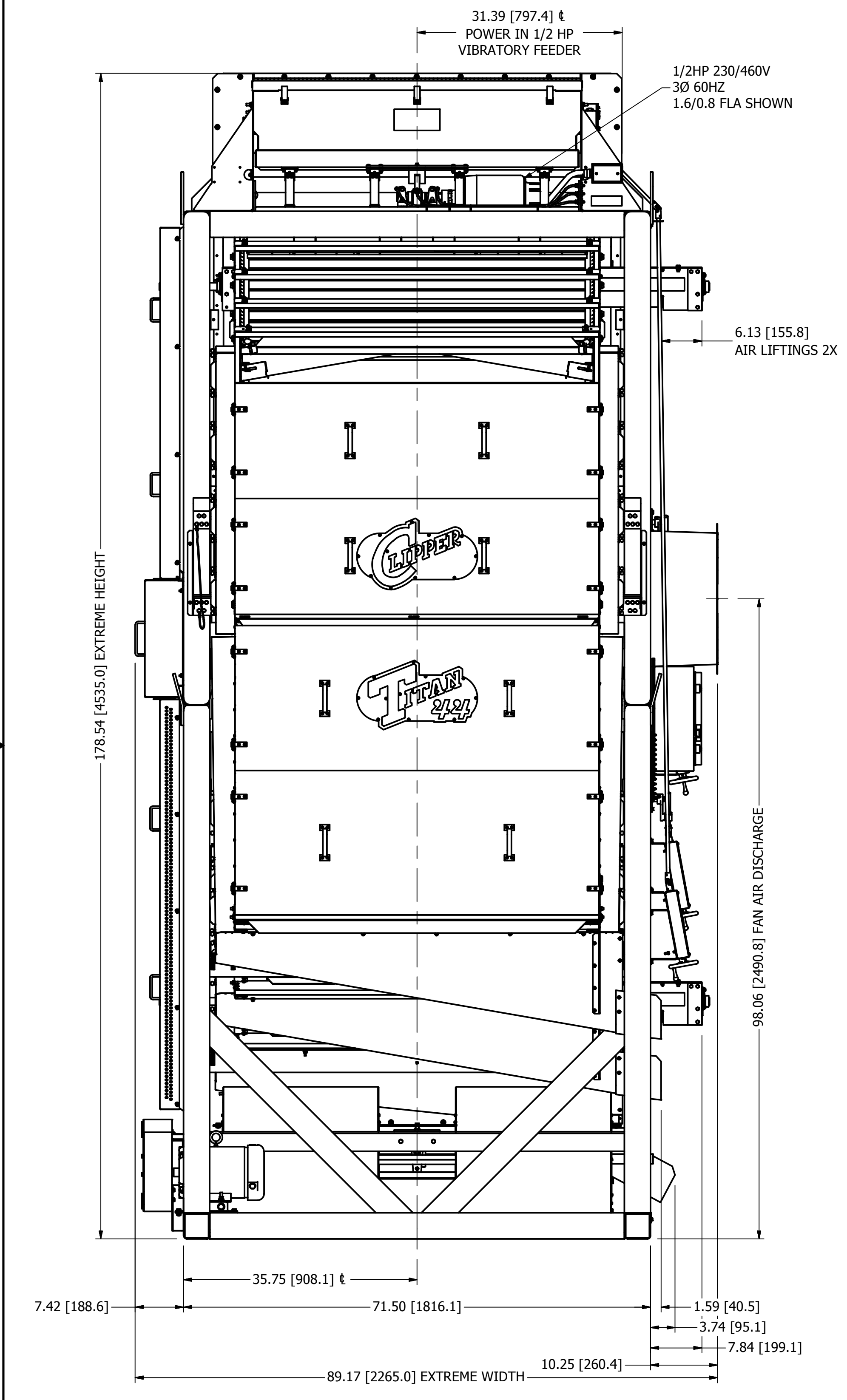
FRONT VIEW
