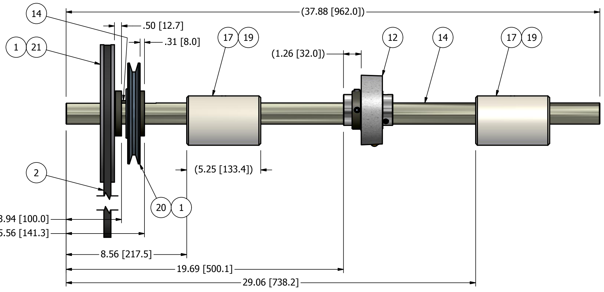
FRONT VIEW: SHAFT ASSEMBLY
