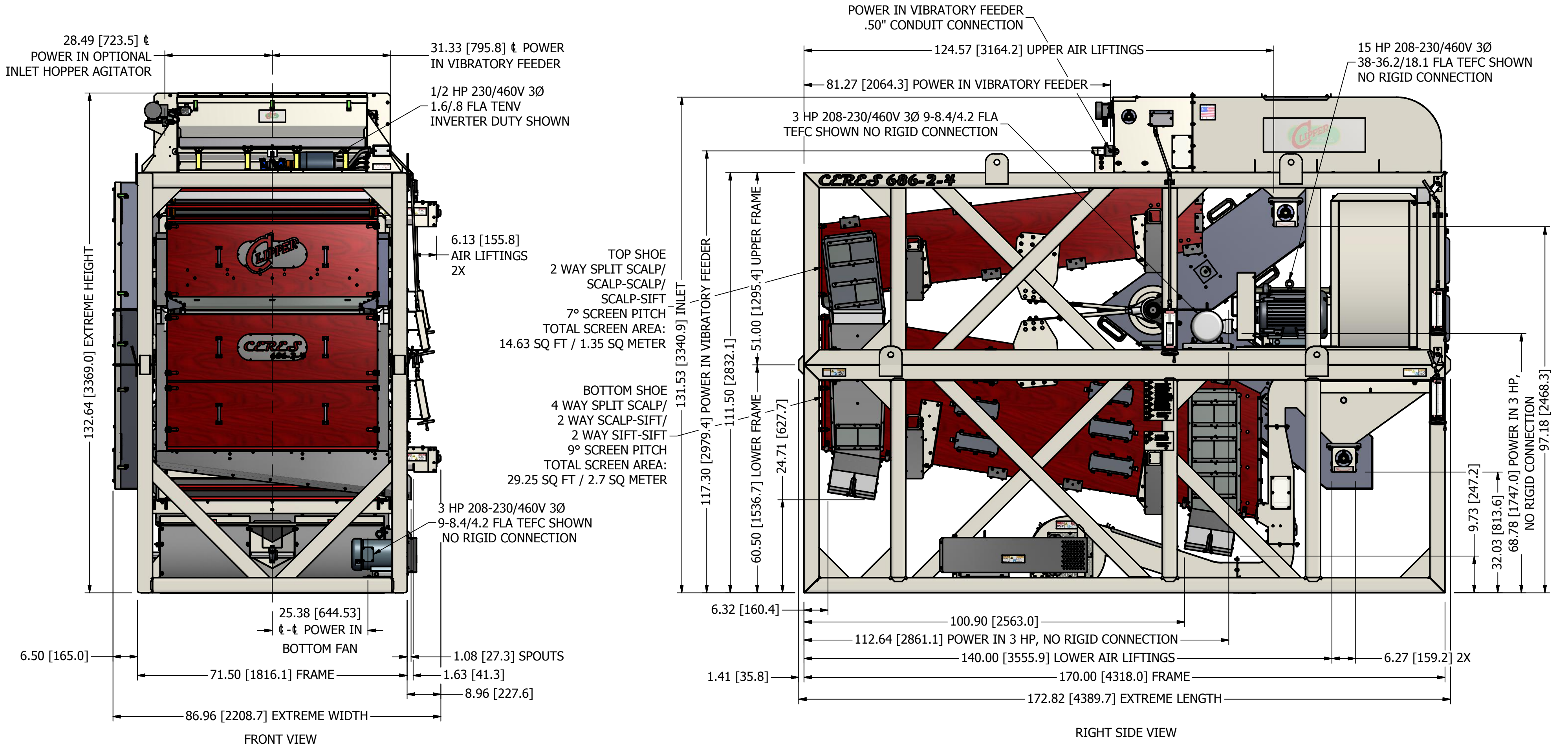
CERES 686-2-4 RH (RIGHT HAND) DISCHARGE ARRANGEMENT SHOWN
